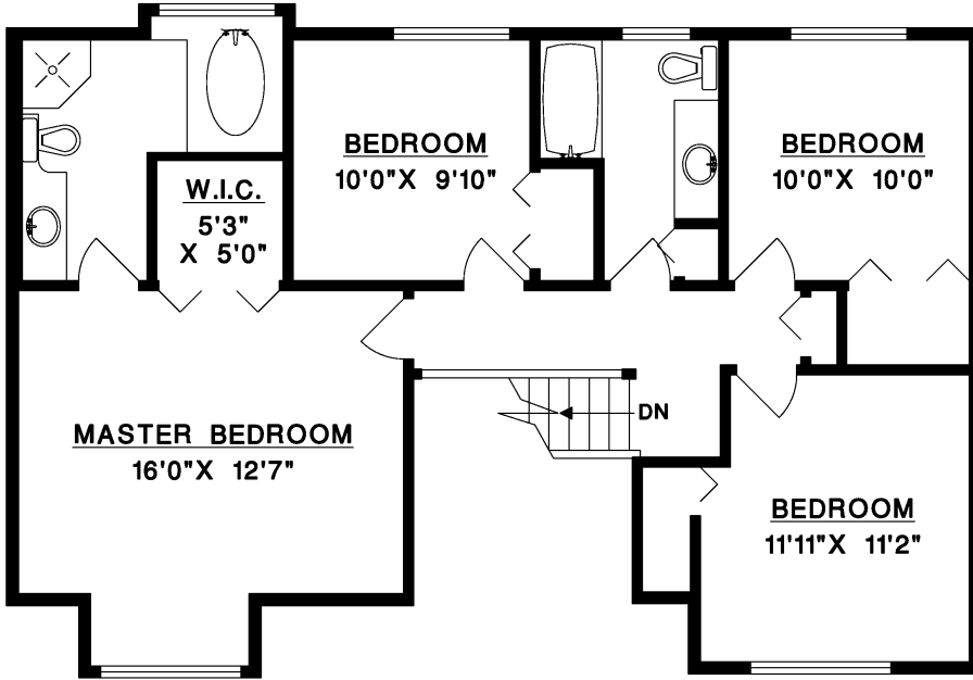
UPPER FLOOR
