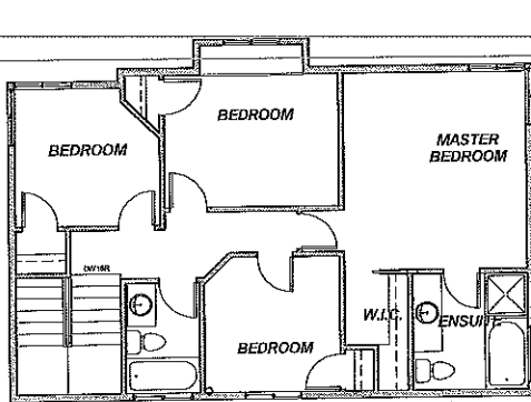
SECOND FLOOR AREA= 859 SF
